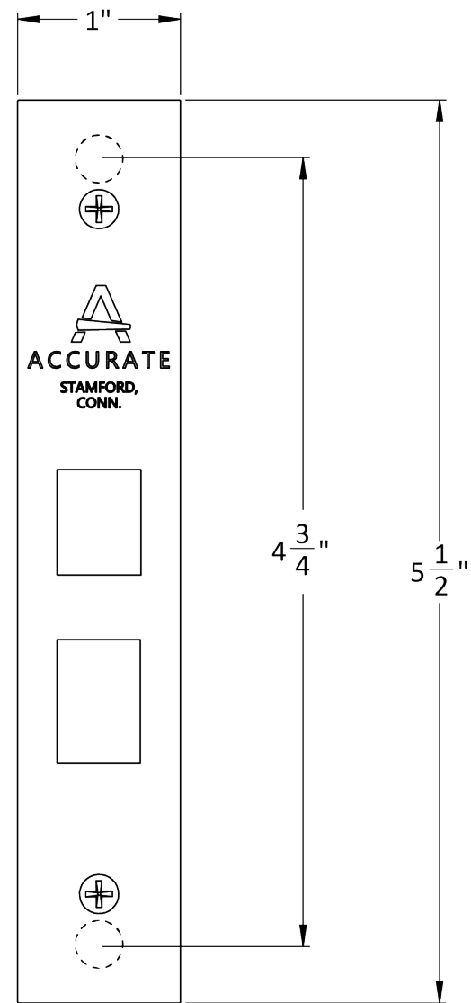
9539MRL PRIVACY MAGNETIC LATCH
