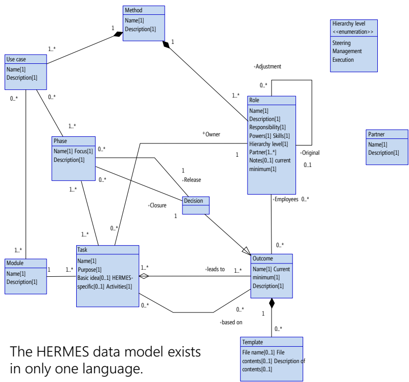
Figure 7: UML diagram of the HERMES data model
