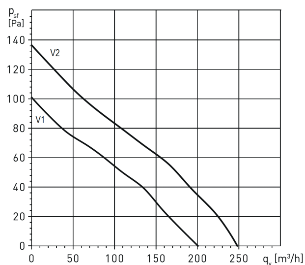
TD 250/100 SILENT
