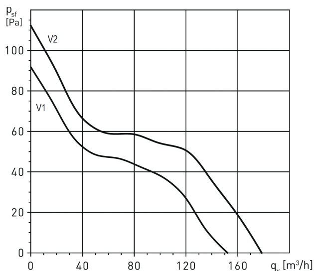
TD 160/100 SILENT
