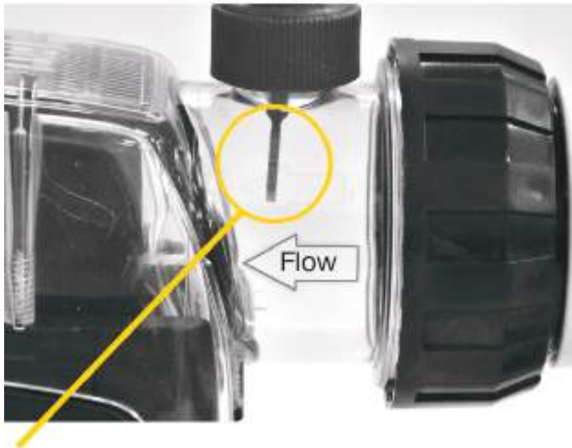
Diagram A CORRECT OPERATION WITH PUMP RUNNING
