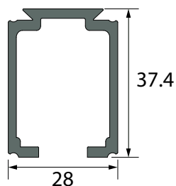
Rail SAF® 120 (11312) (2 - 3 m)
