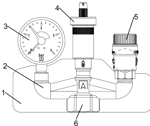
Figure 1: Composants
