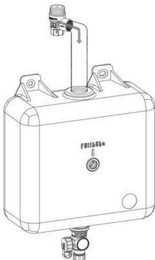
Fig. 2: Installation with discharge line and collector tank for solar liquid
