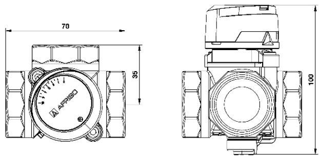
Dimensions (mm)
