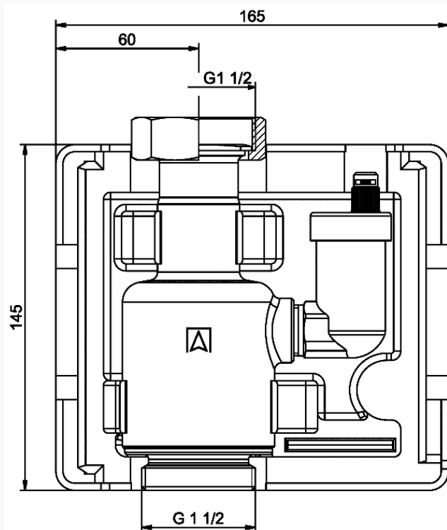
Dimensions (mm)
