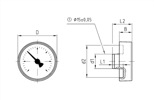
Centre back connection, NG 40
