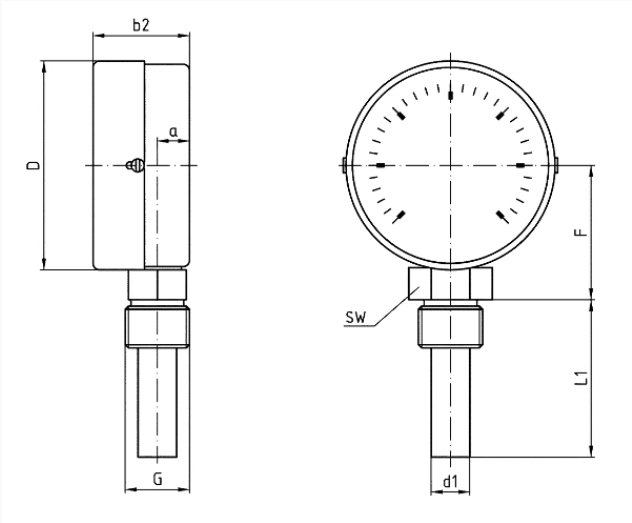
Dimensions (mm)
