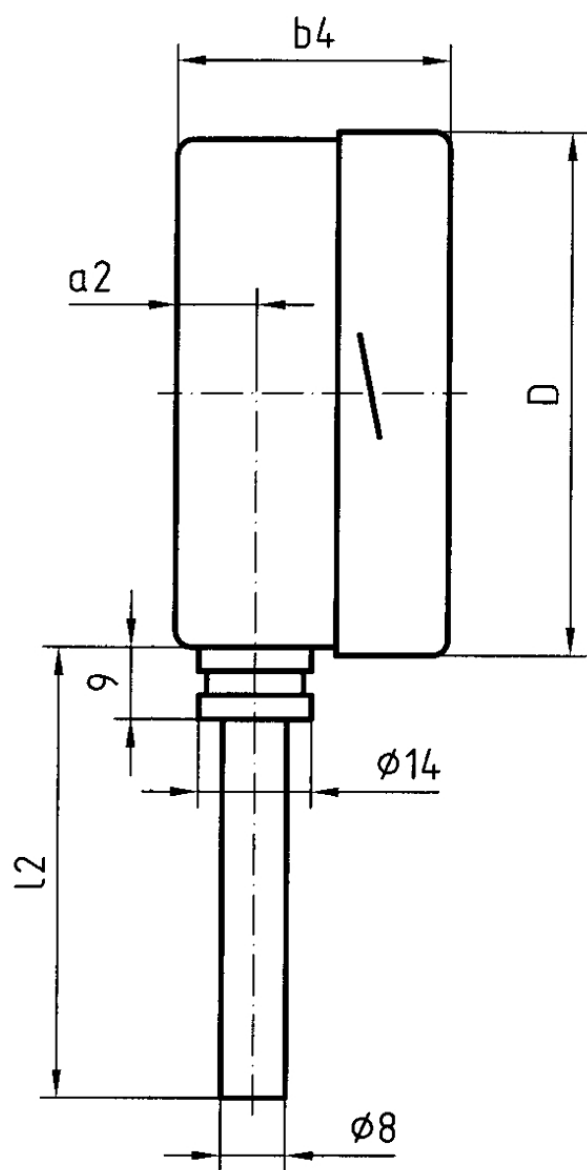
Dimensions (mm)
