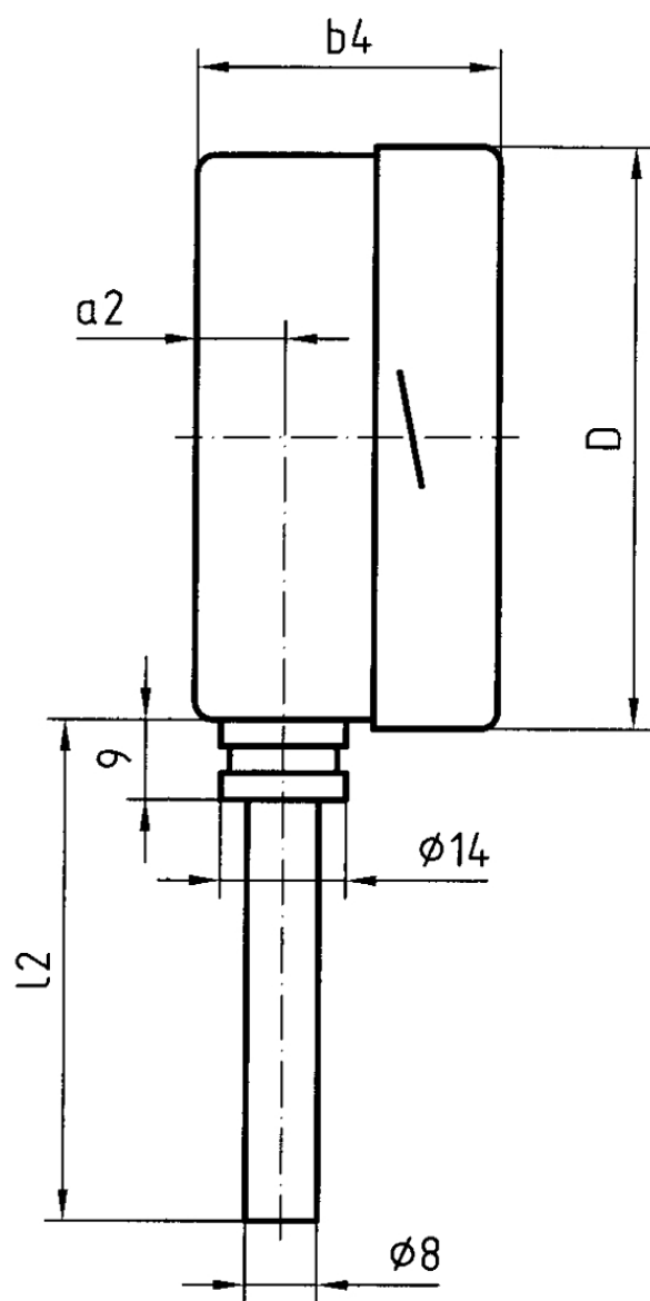
Dimensions (mm)
