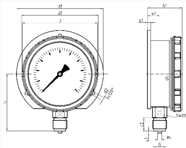
Dimensions (mm)
