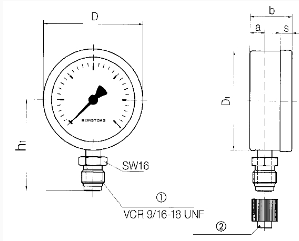
Bottom connection, 9/16-18 UNF, with pressure screw
