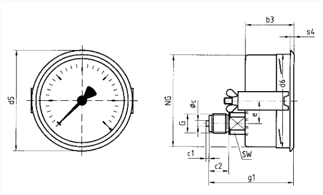
Dimensions (mm)
