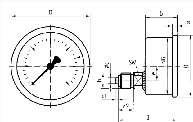
NG 50 – bottom back connection
