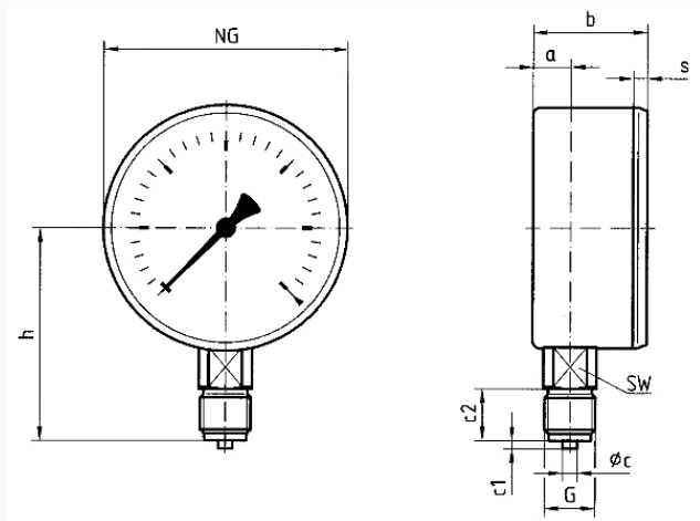
Bottom connection
