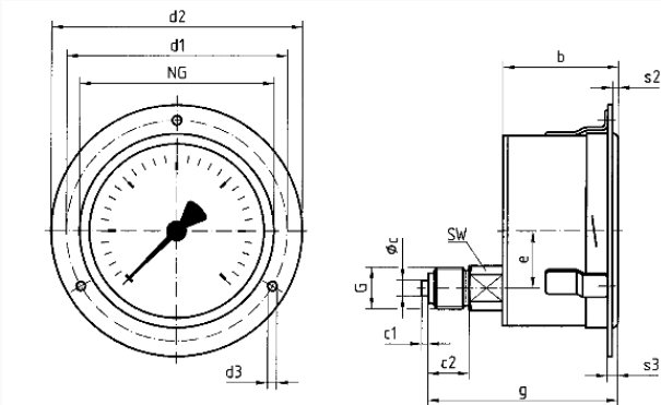
NG 63 – bottom back connection, 3-hole fixing, panel mounting bezel
