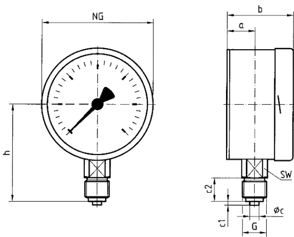
Dimensions (mm)
