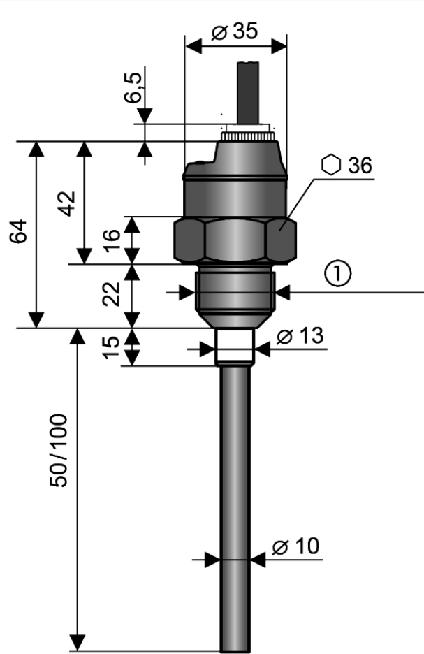
CapFox® ENT 21 MK - 05/10 compact probe with PPS partial insulation
