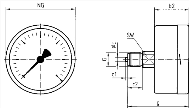
Dimensions (mm)
