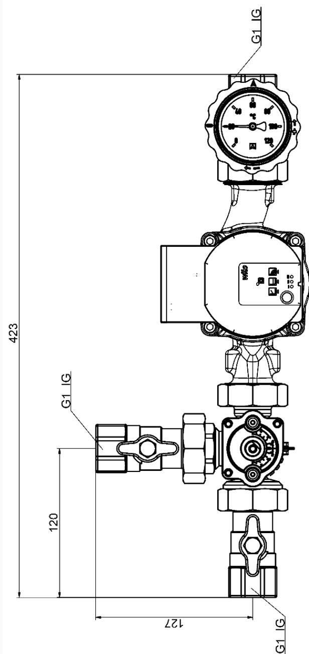
Dimensions (mm)
