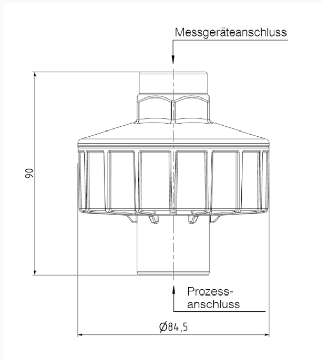
Dimensions (mm)
