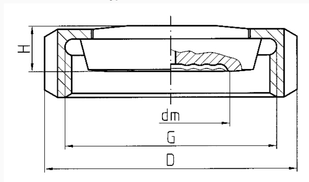
Tapered socket DIN 11851 type D/DIN 11887 type B with grooved union nut DIN 11851 type F
