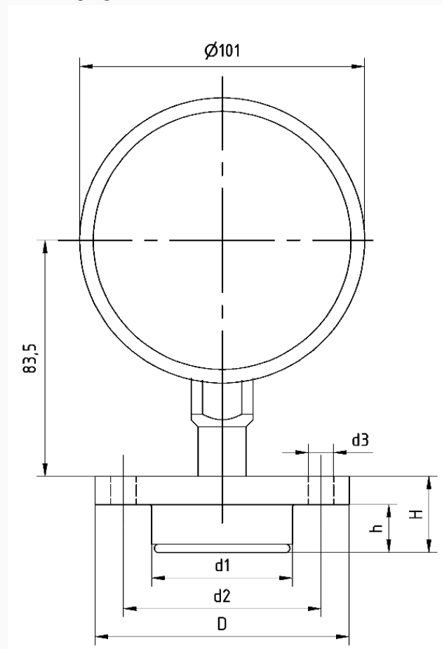
Pressure gauge NG 100 with MD 56
