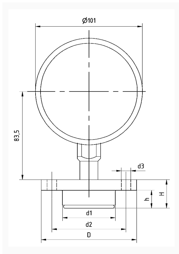
Pressure gauge NG 100 with MD 56
