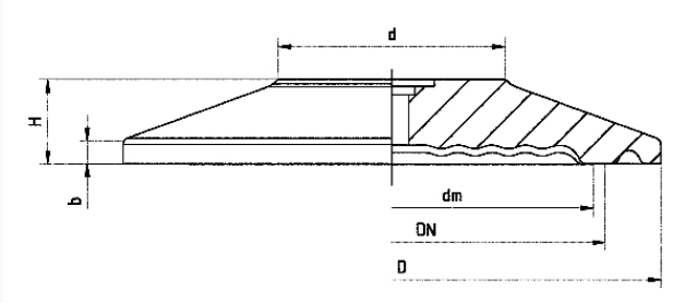
Type MD 60 - clamp connection 1"-2½", ISO 2852
