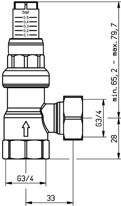
Dimensions (mm)
