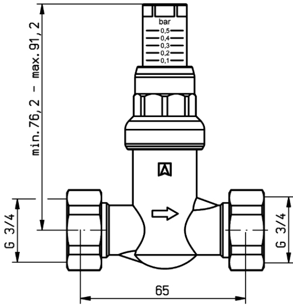
Dimensions (mm)
