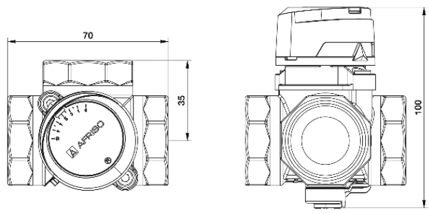
Dimensions (mm)
