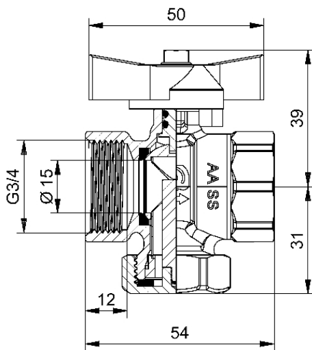
Dimensions (mm)
