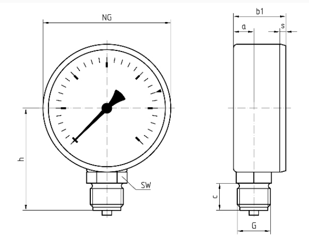
RF 80/HY 80/HZ 80 – bottom connection
