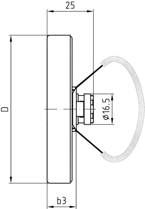
Dimensions (mm)
