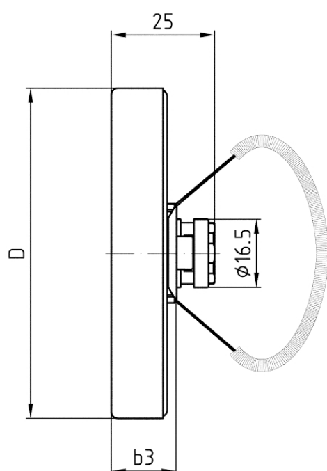
centre back connection, with fastening springs
