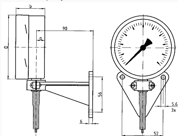
Version with capillary and wall bracket
