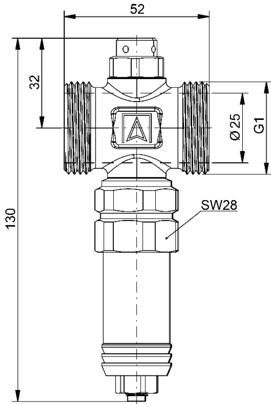
Dimensions (mm)
