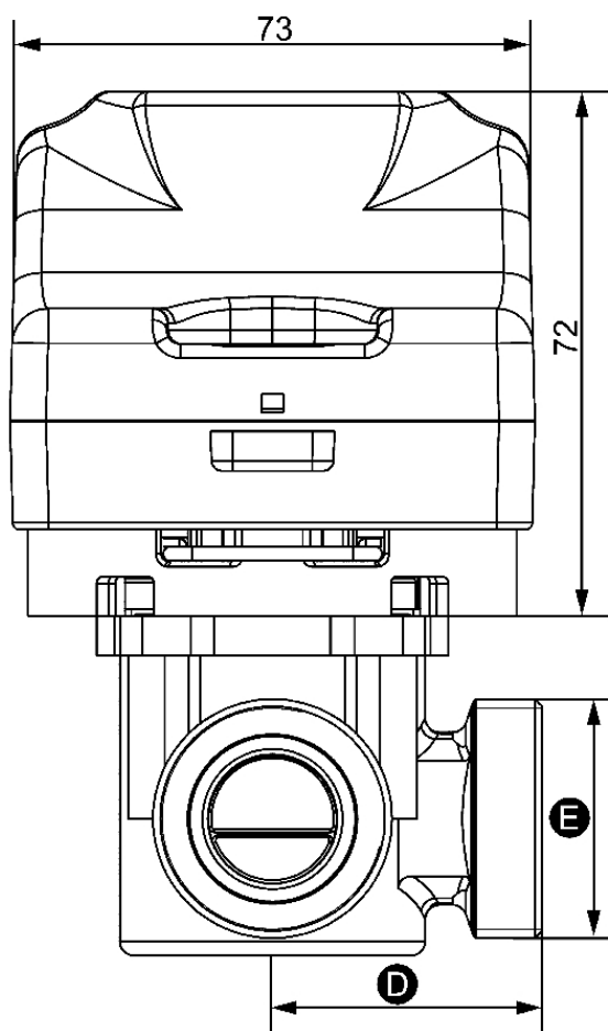
Dimensions (mm)
