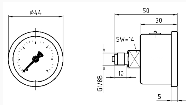
Dimensions (mm)
