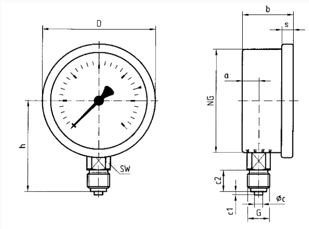
Dimensions (mm)
