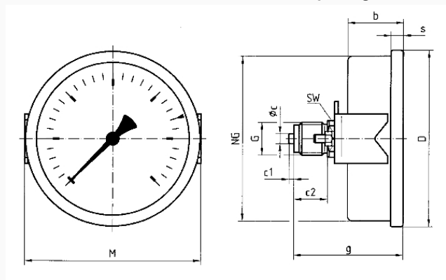
Dimensions (mm)
