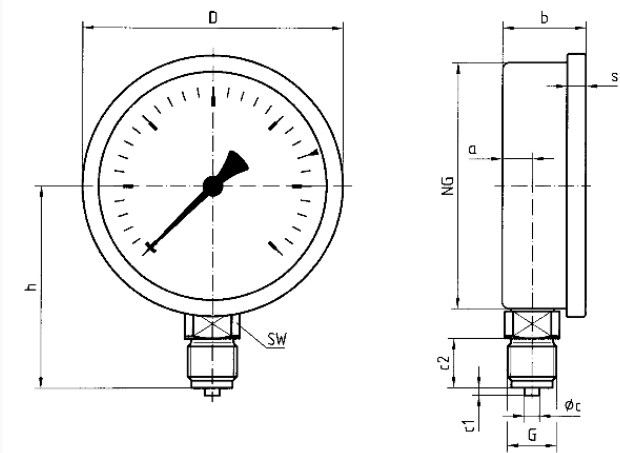
Dimensions (mm)
