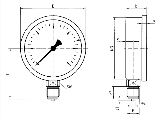
Dimensions (mm)
