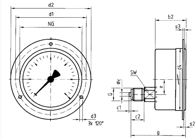
Dimensions (mm)
