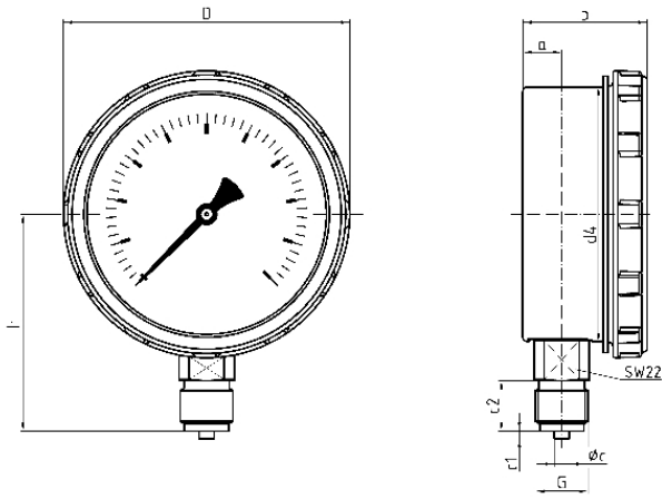
Dimensions (mm)
