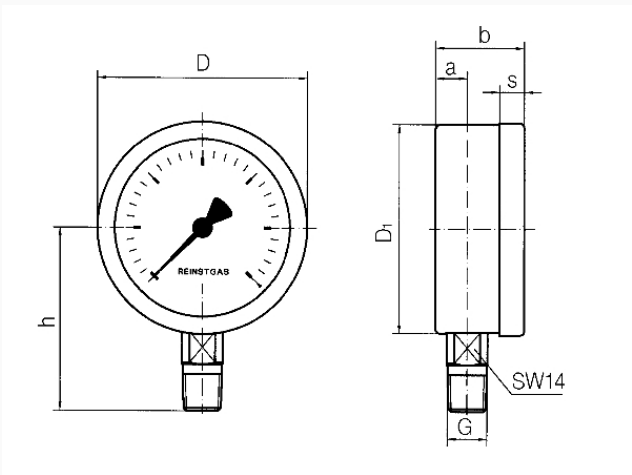
Bottom connection, 1/4-18 NPT
