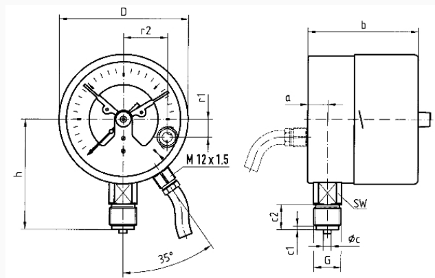
Bottom connection
