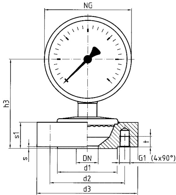
Dimensions (mm)
