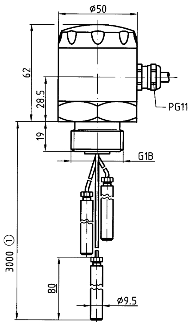
Flexible probe LSE 23
