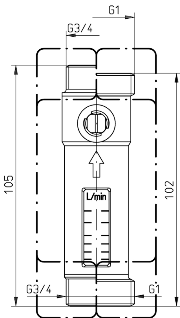
DFM 15-2M, male thread x male thread
