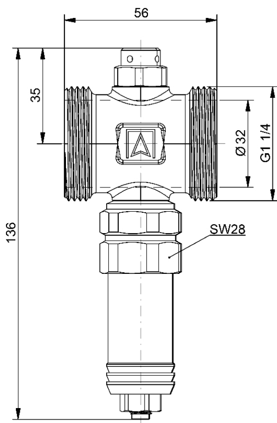
Dimensions (mm)
